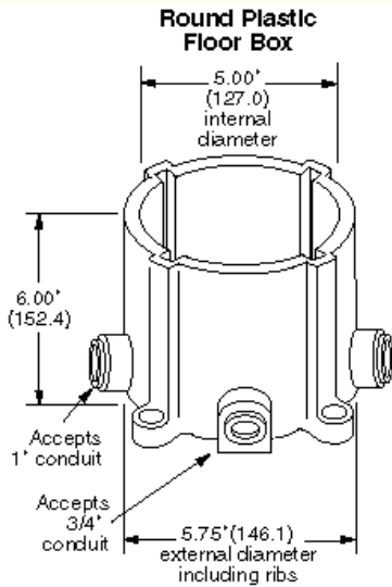
Plastic Floor Box, Round
