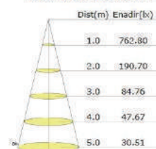
Illuminance at a Distance
