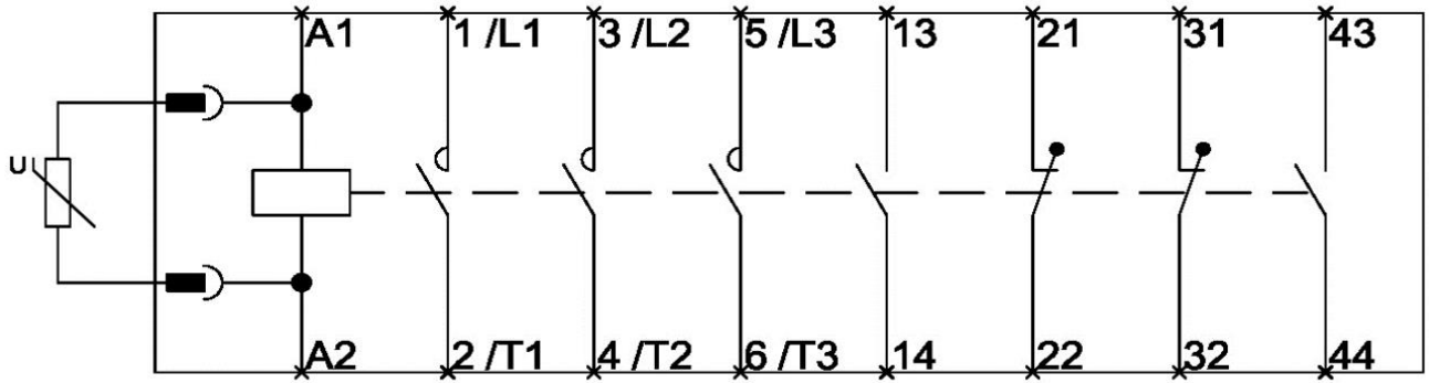
LENOOF G & H Wiring Diagram
