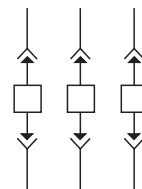
Fig. F U0353F, U0653F Fusible
