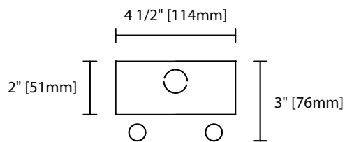
ST2 T5 Cross Section View
