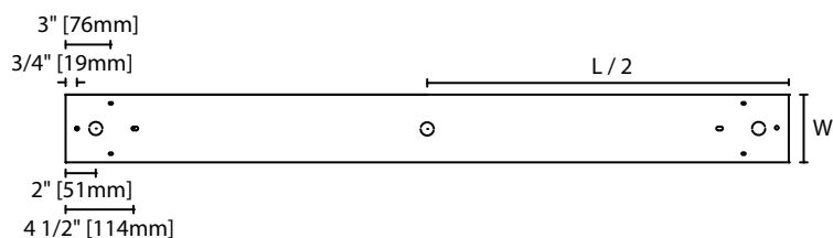
Base View
