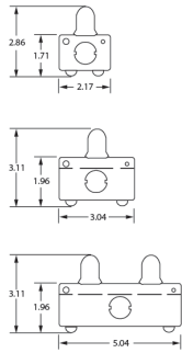
End View
