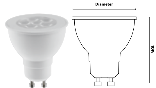
MOL : 2 3/32 in. (53.5 mm) Dia. : 1 15/16 in. (49 mm)
