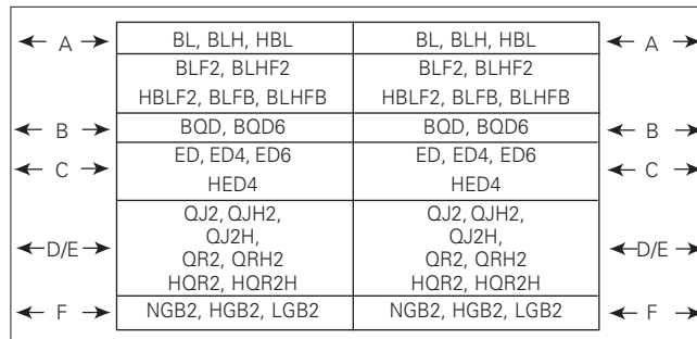
Panel Width 24 in. (610 mm) Branch Breaker Side Gutters
