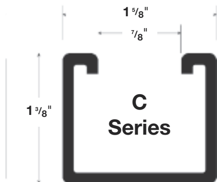
C Series C1200 12 gauge
