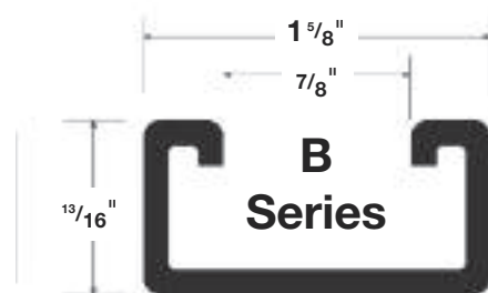
B Series B1200 12 gauge B1400 14 gauge
