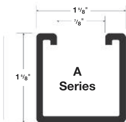
A Series A1200 12 gauge A1400 14 gauge
