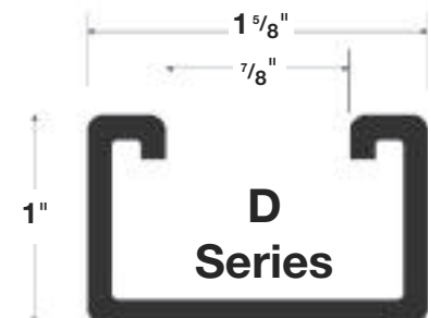
D Series D1200 12 gauge
