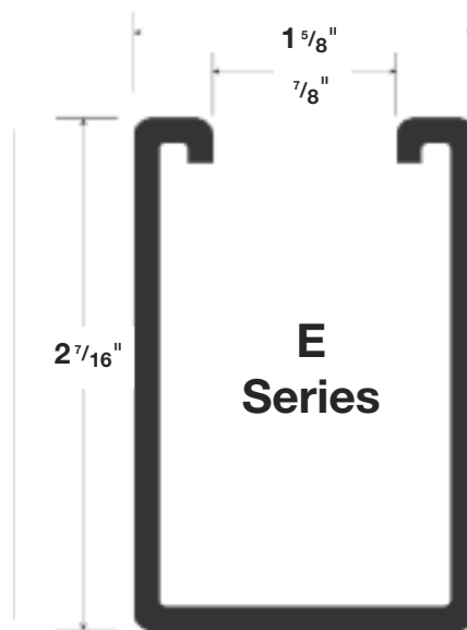
E Series E1200 12 gauge
