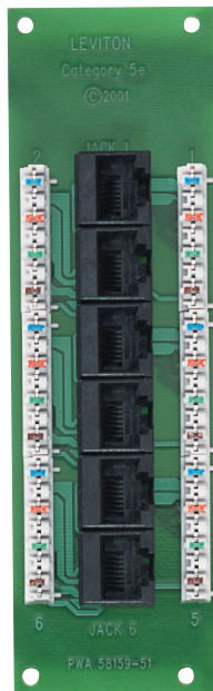
Expansion Board
