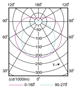
LEDtube 900 mm 10.5 W /840
