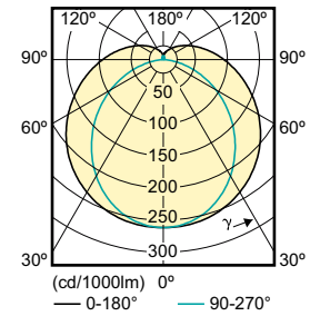
LED InstantFit T8 1200mm 16.5 W, 600mm 8.5 W /840
