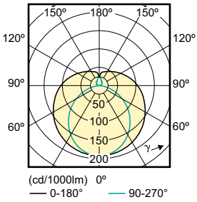
LEDtube 1200mm 17 W
