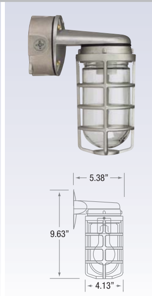
DVBKS100CG Wall Mount
