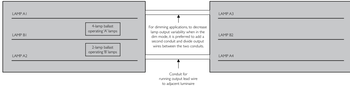
2 BALLAST EXAMPLE
