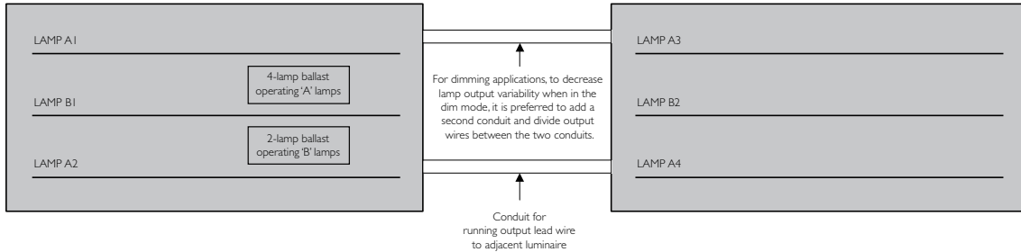
2 BALLAST EXAMPLE
