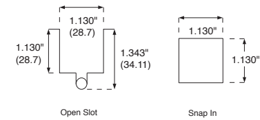
PANEL CUTOUT
