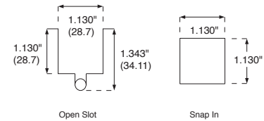
PANEL CUTOUT
