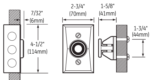
1509-AQN5 Completely Flush Wall Mounted
