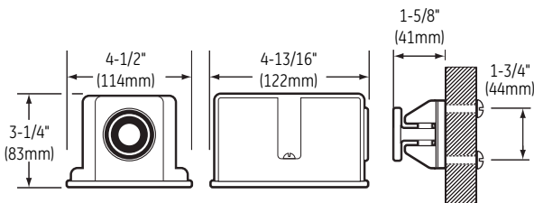
1501-AQN5 Floor Mounted (Single Door)
