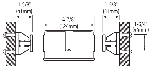
1502-AQN5 Floor Mounted (Double Door)
