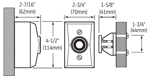
1508-AQN5 Surface Wall Mounted
