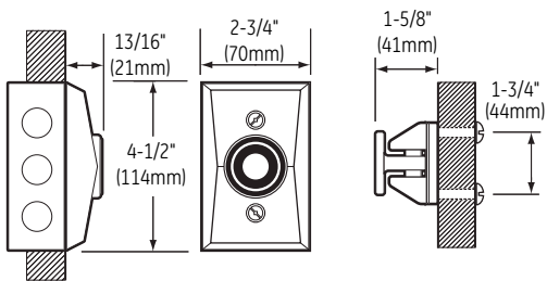
1505-AQN5 Flush Wall Mounted (Short Catch Plate)
