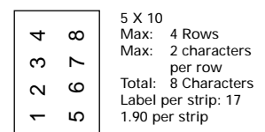
Vertical 8WA8847-Z2
