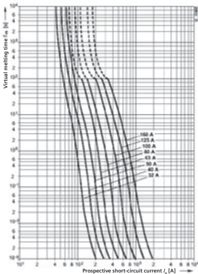
Fig. 5.5.4 – Time/current characteristic curves for SITOR gR and aR fuse links
