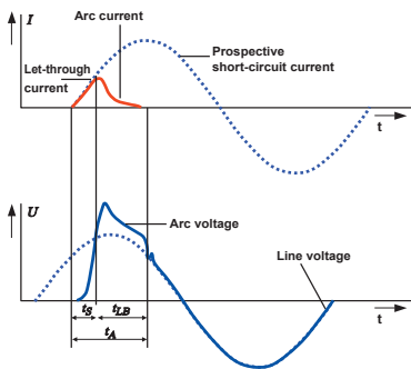
Fig. 4.1.3 – Short-circuit current limiting
