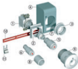
Fig. 3.1.6 – DIAZED® system components
