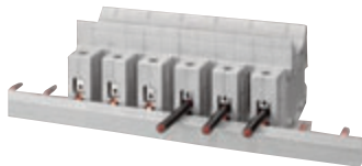
Fig. 3.3.7 – NEOZED fuse base on busbar
