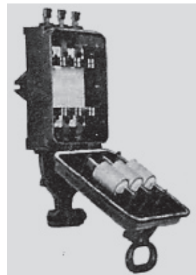
Fig. 2.8 – Plug-in porcelain car- tridges (1910) 10)
