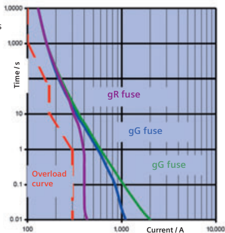
Fig. 5.5.2 – gG, gS, and aR characteristic curves with overload curve
