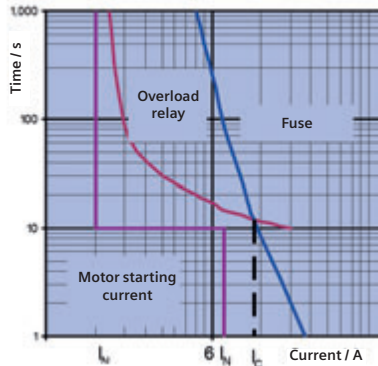
Fig. 5.4.2 – Selection of motor protection fuses
