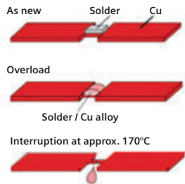
Fig. 4.1.5 – Solder reaction at overload tripping
