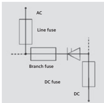
Fig. 5.5.1 – Semiconductor protection, circuit diagram
