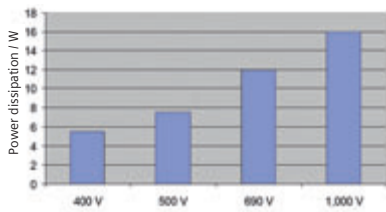
Fig. 4.5.4 – power dissipation of 100 A gG fuse links
