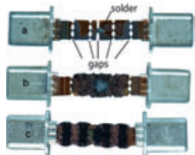
Fig. 4.1.4 – LV HRC fuse element a) new b) after overload tripping c) after short-circuit tripping
