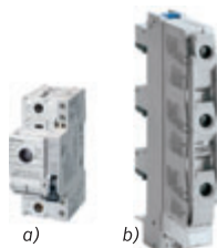
Fig. 3.6.4 – a) MINIZED switch disconnectors D02 with auxiliary switch for remotely monitoring the switch position b) NEOZED bar-mounting switch disconnector D02
