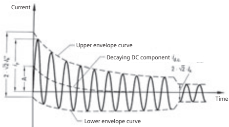
Fig. 4.3.5 – Short-circuit current characteristic in a three-phase system
