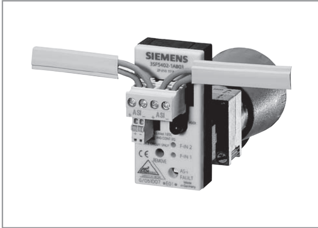
EMERGENCY-STOP mushroom push button with F adapter for bus connection
