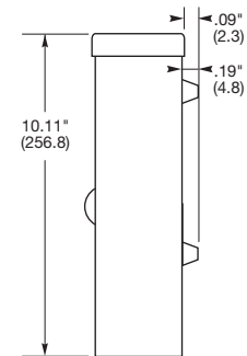
SIDE VIEW HBL16R90/HBL16R92D/HBL16R93D
