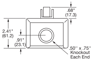
END VIEW HBL1370/HBL1372D/HBL1379D
