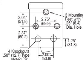
BACK VIEW HBL13R89D / HBL13R90 HBL13R92D
