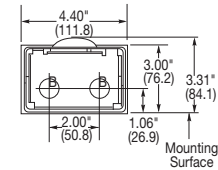
END VIEW HBL13R89D / HBL13R90 HBL13R92D
