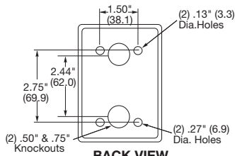
BACK VIEW HBL1370/HBL1372D/HBL1379D
