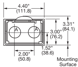
END VIEW HBL16R90/HBL16R92D/HBL16R93D
