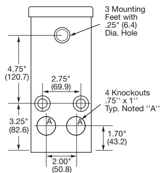
BACK VIEW HBL16R90/HBL16R92D/HBL16R93D
