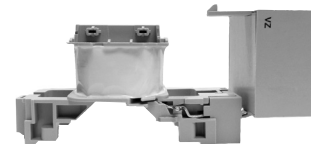
36V...220V Electronic DC coil with Back Pack ③
